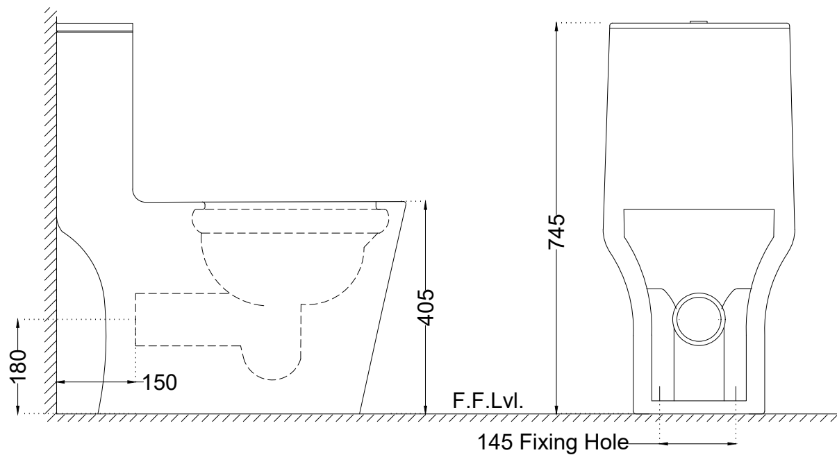
SIDE VIEW
