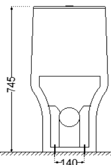
BACK VIEW
